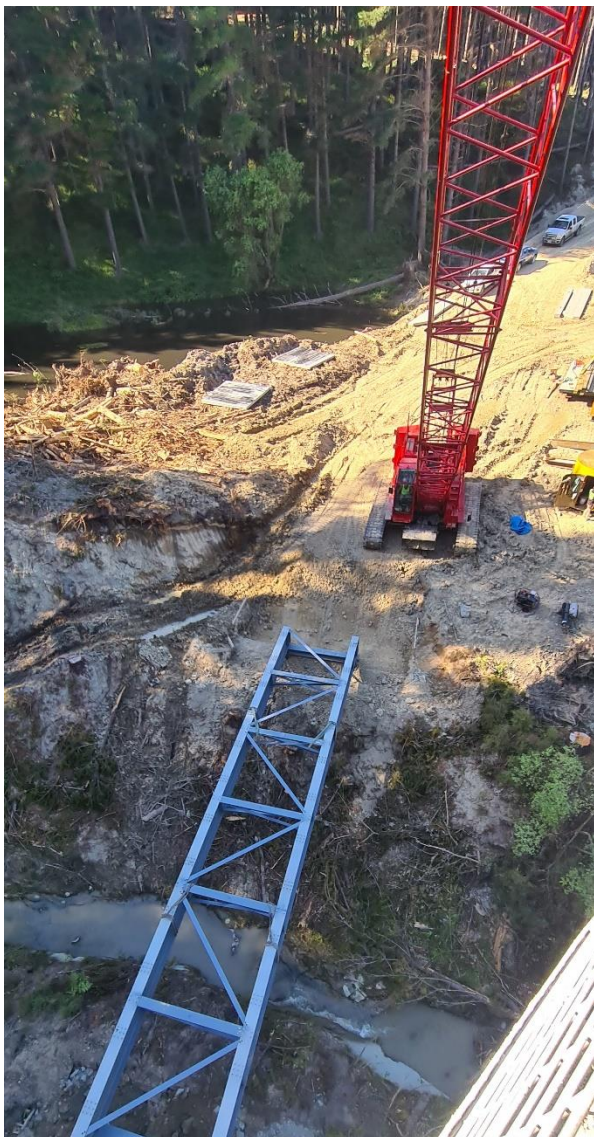
Photo 4: Looking down on the bridge site from the crane cage.
